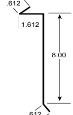
Reglet Flashing (not shown)
