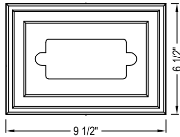
HORIZONTAL RECESSED MOUNT WATER MANAGEMENT LOCKING POSITIONS 7/16", 11/16", 15/16"
