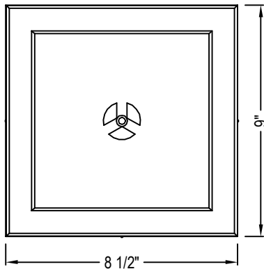
MOUNTMASTER WATER MANAGEMENT LOCKING POSITIONS 7/16", 11/16", 15/16"
