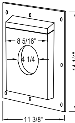
STURDIMOUNT® UNIVERSAL MOUNT
