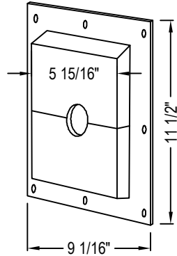
STURDIMOUNT® SPLIT MOUNT
