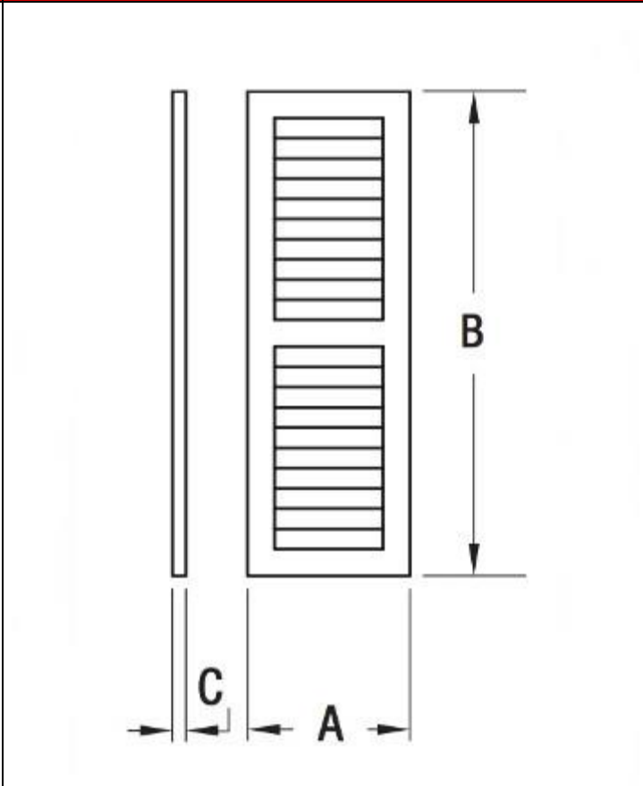
Center Rail Louvered Shutter Profile
